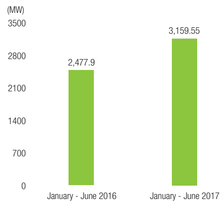
Wind Power Consolidated Installed Capacity
